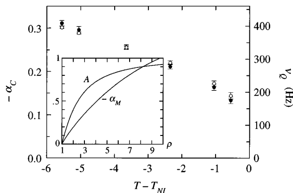
FIG. 17. Temperature variation of the water diffusion anisotropy \alpha_C (●) and the water ^2\text{H} quadrupole splitting \nu_Q (○) in the nematic phase of the \phi=0.227 sample. The bars represent the experimental error. The inset shows the variation of the shape factor A and the micelle-frame diffusion anisotropy \alpha_M with the aspect ratio \rho of an oblate spheroid ( \phi=0.227 , n=6 , D_1/D_0=0.4 ).
