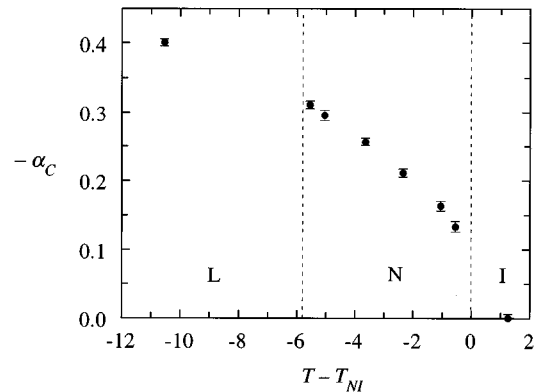
FIG. 9. Temperature variation of the anisotropy \alpha_C of the water self-diffusion tensor for the \phi=0.227 sample in the lamellar (L), nematic (N), and isotropic (I) phases. The bars represent the experimental error.
