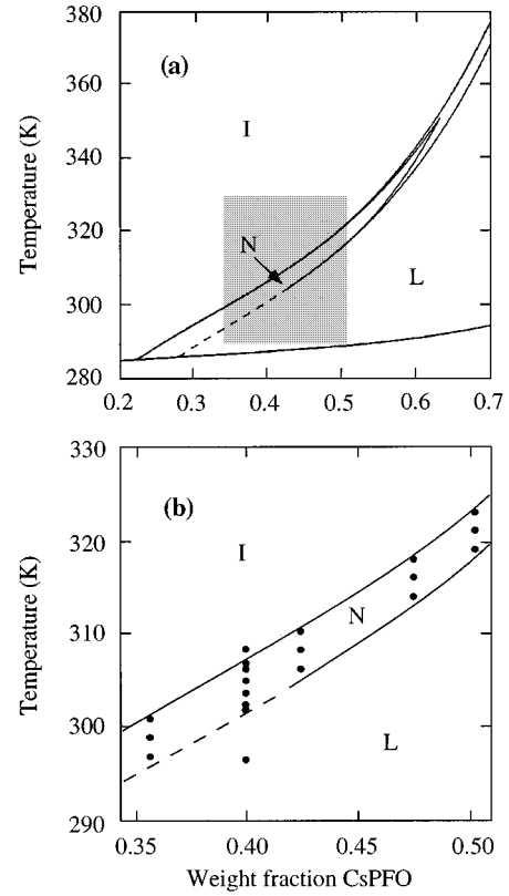
FIG. 1. (a) Partial phase diagram for the CsPFO-D 2 O system, taken from Ref. [4], showing the isotropic-to-nematic and nematic-to-lamellar transition curves and the solubility curve. Along the dashed curve, a two-phase region has so far not been detected [4]. (b) Enlargement of the shaded area in (a), showing the 20 investigated sample points.
