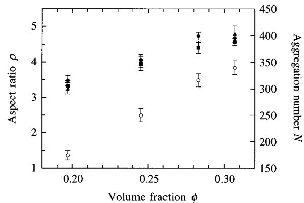
FIG. 14. Variation of the micellar aspect ratio \rho derived from D_{\text{iso}}/D_0 , with the micelle volume fraction \phi for four nematic samples at relative temperatures, T-T_{NI} = -0.5 K (●), -2.5 K (■), and -4.5 K (▲). The micellar aggregation number N (○) was calculated from the average \rho assuming a minor semiaxis of 11 \text{ \AA} . The bars represent the propagated experimental error.
