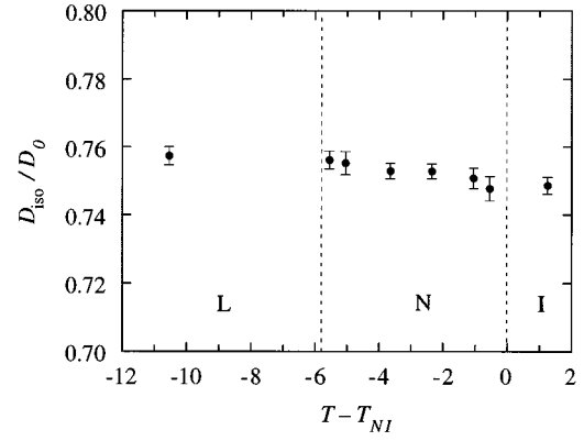
FIG. 8. Temperature variation of the relative, isotropically averaged, water self-diffusion coefficient, D_{\text{iso}}/D_0 , for the \phi=0.227 sample in the lamellar (L), nematic (N), and isotropic (I) phases. The bars represent the experimental error.
