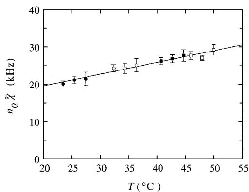
FIG. 16. Temperature variation of the quantity n_Q\bar{\chi} derived from the water ^2\text{H} quadrupole splitting and the \rho and S values obtained from the diffusion data. The symbols refer to samples of different volume fraction, \phi=0.197 (●), 0.244 (○), 0.283 (■), and 0.307 (□). The bars represent the propagated experimental error.
