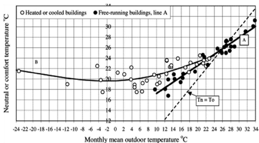
Fig. 3.2.2 Neutral temperature vs. outdoor temperature for active and passive (free-running) buildings (from Nicol sited in Emmanuel 2005).
